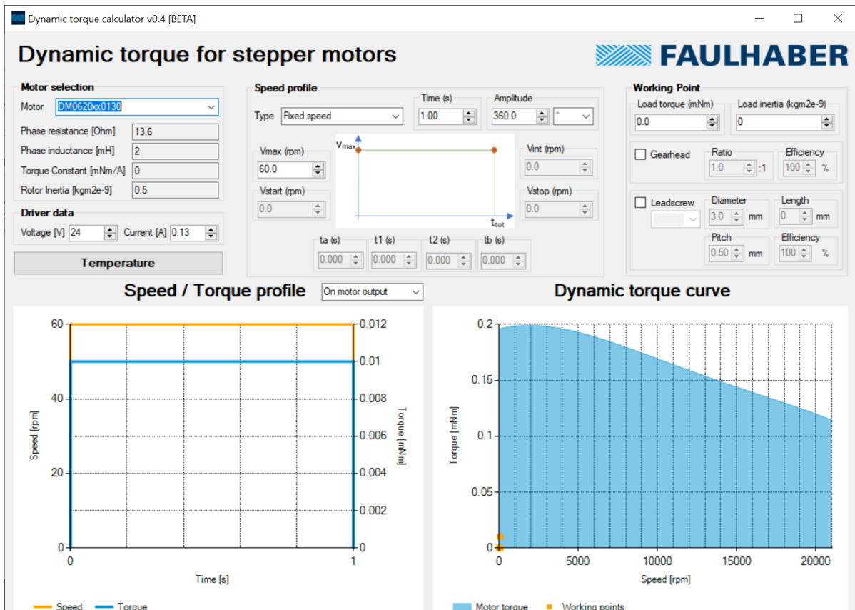
Figure 4 : Interface of the Dynamic torque calculator
