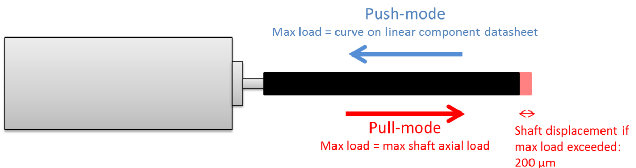
Figure 5 - limits for axial forces the motor can overcome
